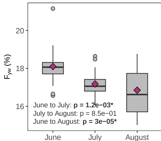
Prior: 0.153/0.847
