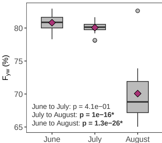
Prior: 0.8/0.2
