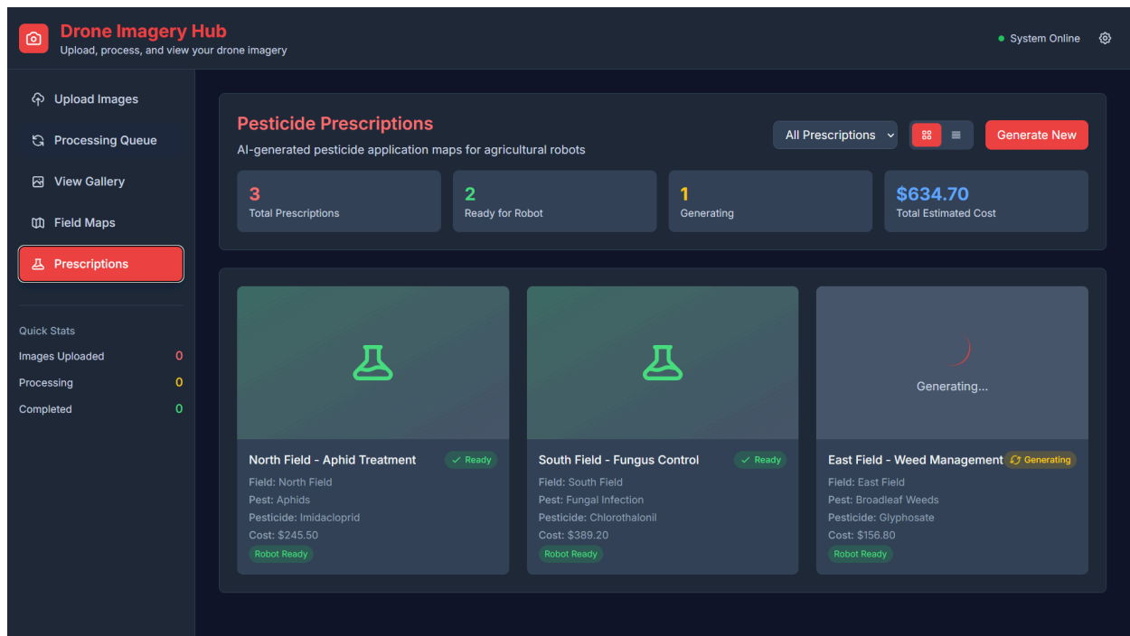
Figure 7 Prescription UI
