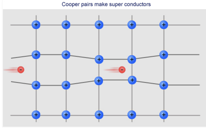
Figure 4: Illustration of how deformation of the ion lattice mediates attraction between electrons, leading to the formation of Cooper pairs and thus superconductivity, taken from [12]
