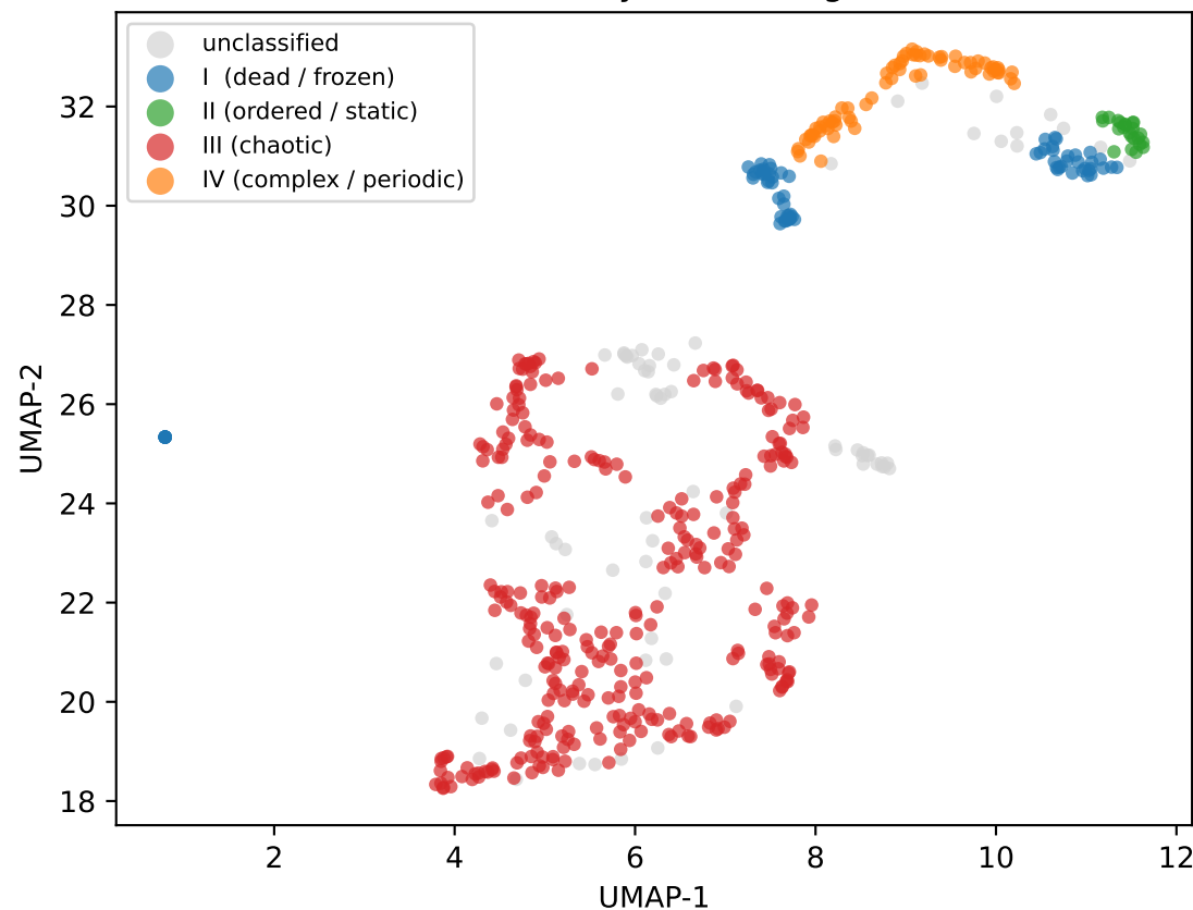
(a) Wolfram dynamical regimes
