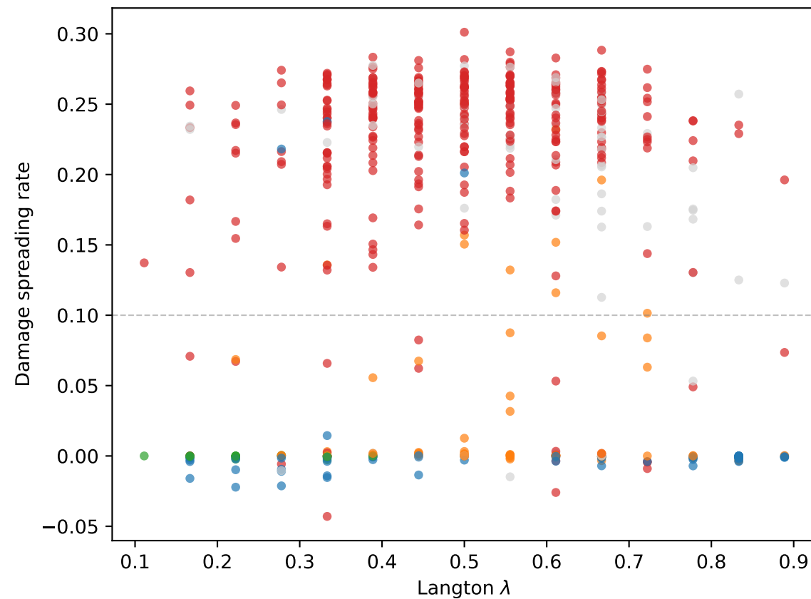
(b) \lambda vs Lyapunov-like exponent
