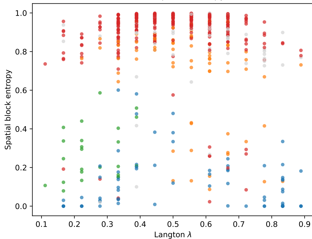
(c) \lambda vs spatial entropy
