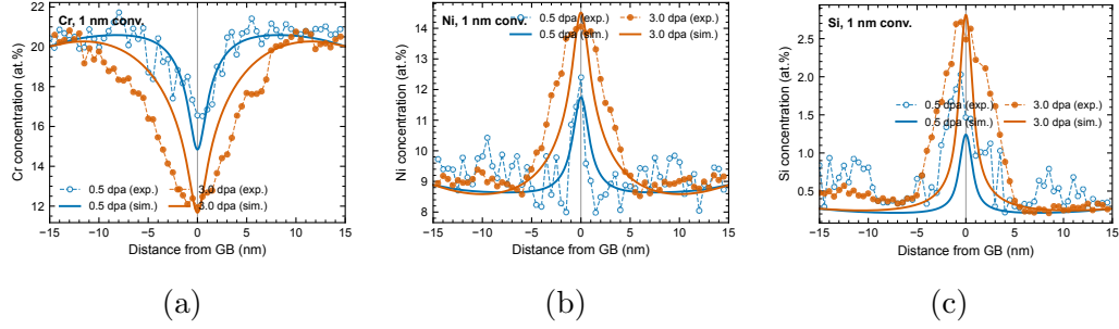
Figure 1: Calculated and measured grain-boundary composition profiles after irradiation to 0.5 and 3.0 dpa: (a) Cr, (b) Ni, (c) Si. Solid lines are calculated profiles convolved with a 1 nm Gaussian; open and filled symbols are the measurements of at 0.5 and 3.0 dpa respectively.
