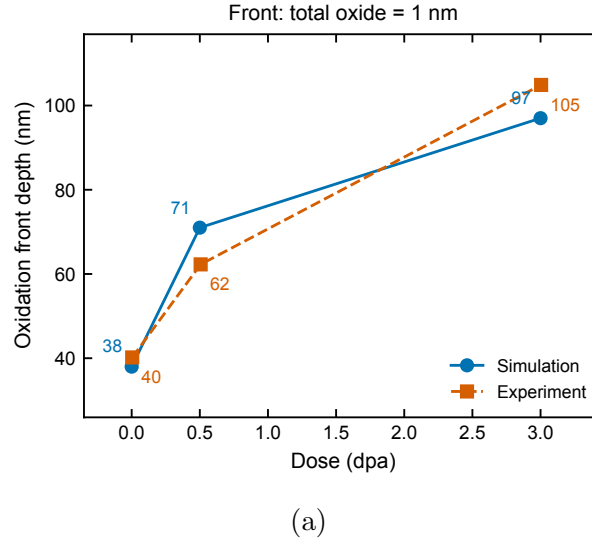
Figure 2: Oxidation front depth as a function of dose, taken at a total oxide thickness of 1 nm. Measurements from deng are those used to calibrate the oxidation parameters.
