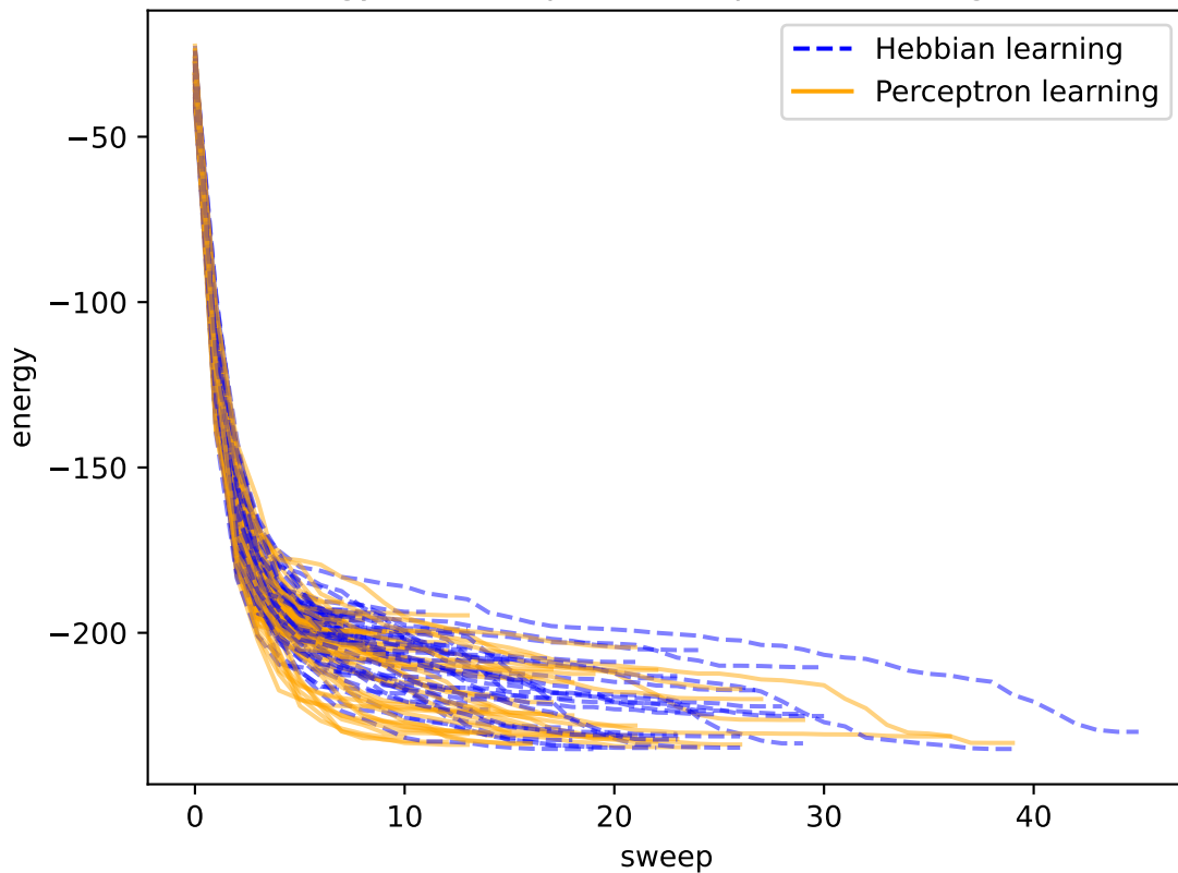
Energy vs. Sweep for Perceptron Learning Rule
