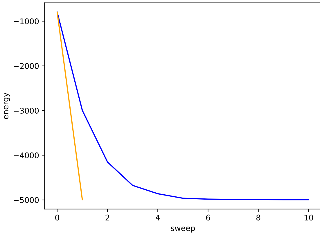
Energy vs. Sweep for Hebbian Learning Rule
