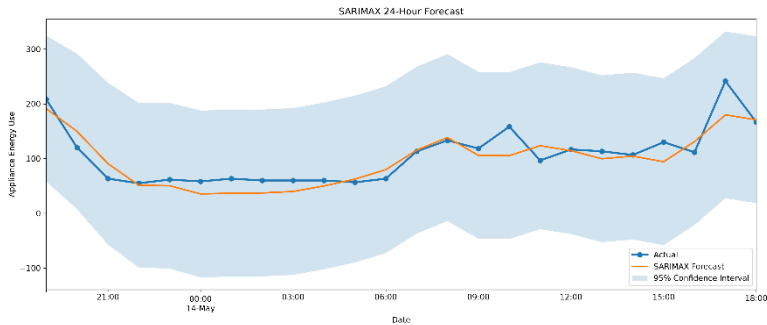
Figure 7: Comparison of observed and predicted hourly appliance energy consumption using the final SARIMAX model with 95% prediction intervals over the 24-hour forecast horizon.
