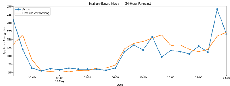
Figure 9:Comparison of observed and predicted hourly appliance energy consumption using the HistGradientBoosting feature-based forecasting model over the 24-hour prediction horizon
