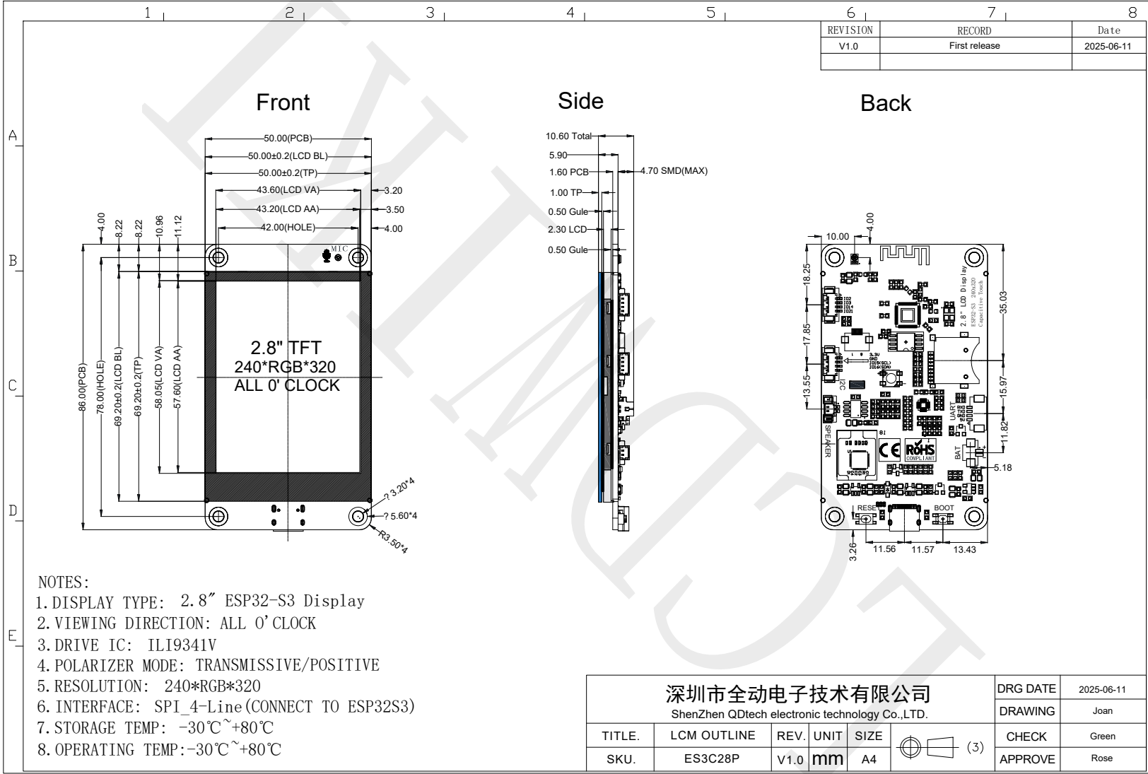
Figure 5.1 ES3C28P Outline Drawing
