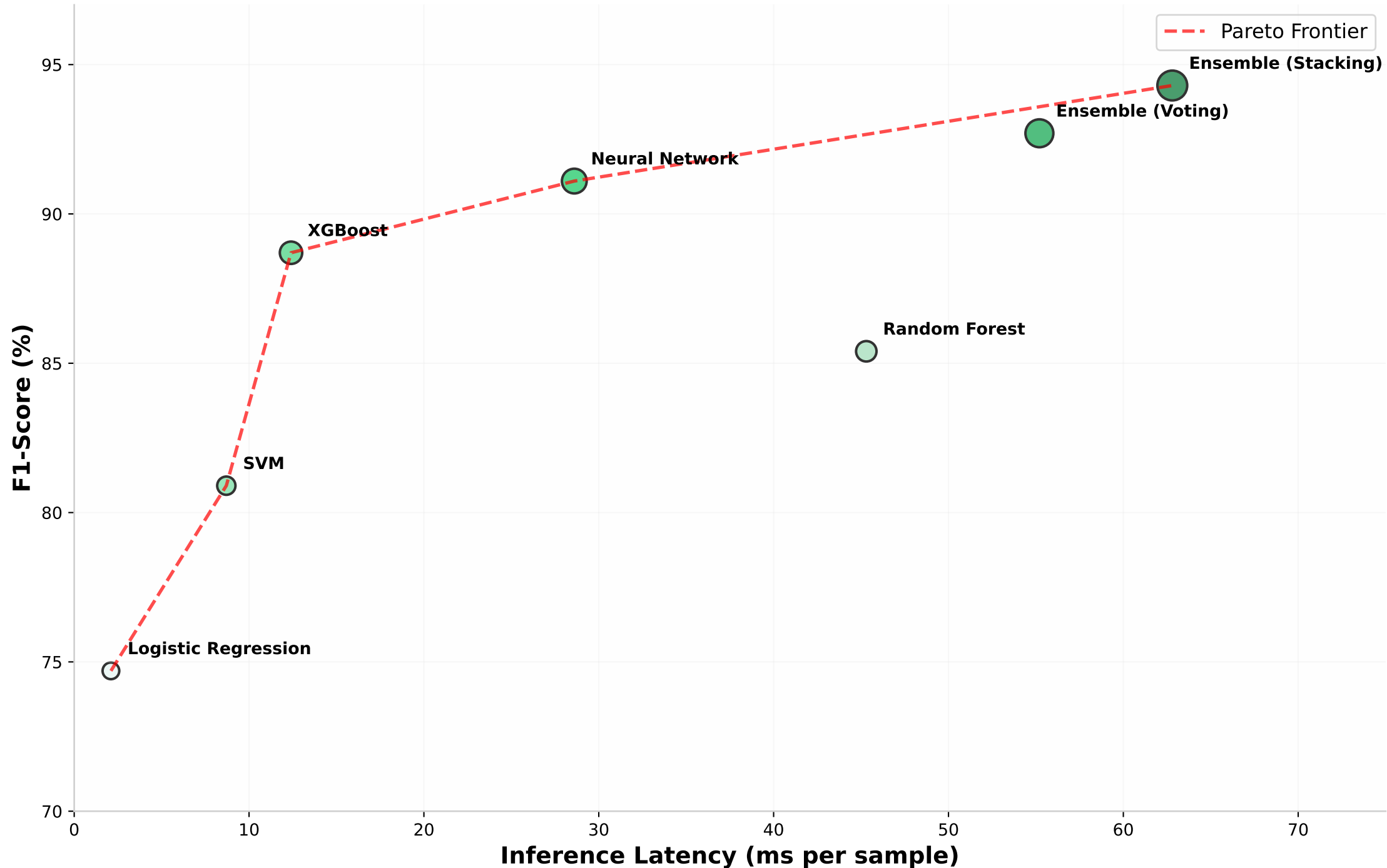
Figure 1.2 — Performance-Efficiency Trade-off Health Risk Prediction Models on Global Blood Test Dataset
