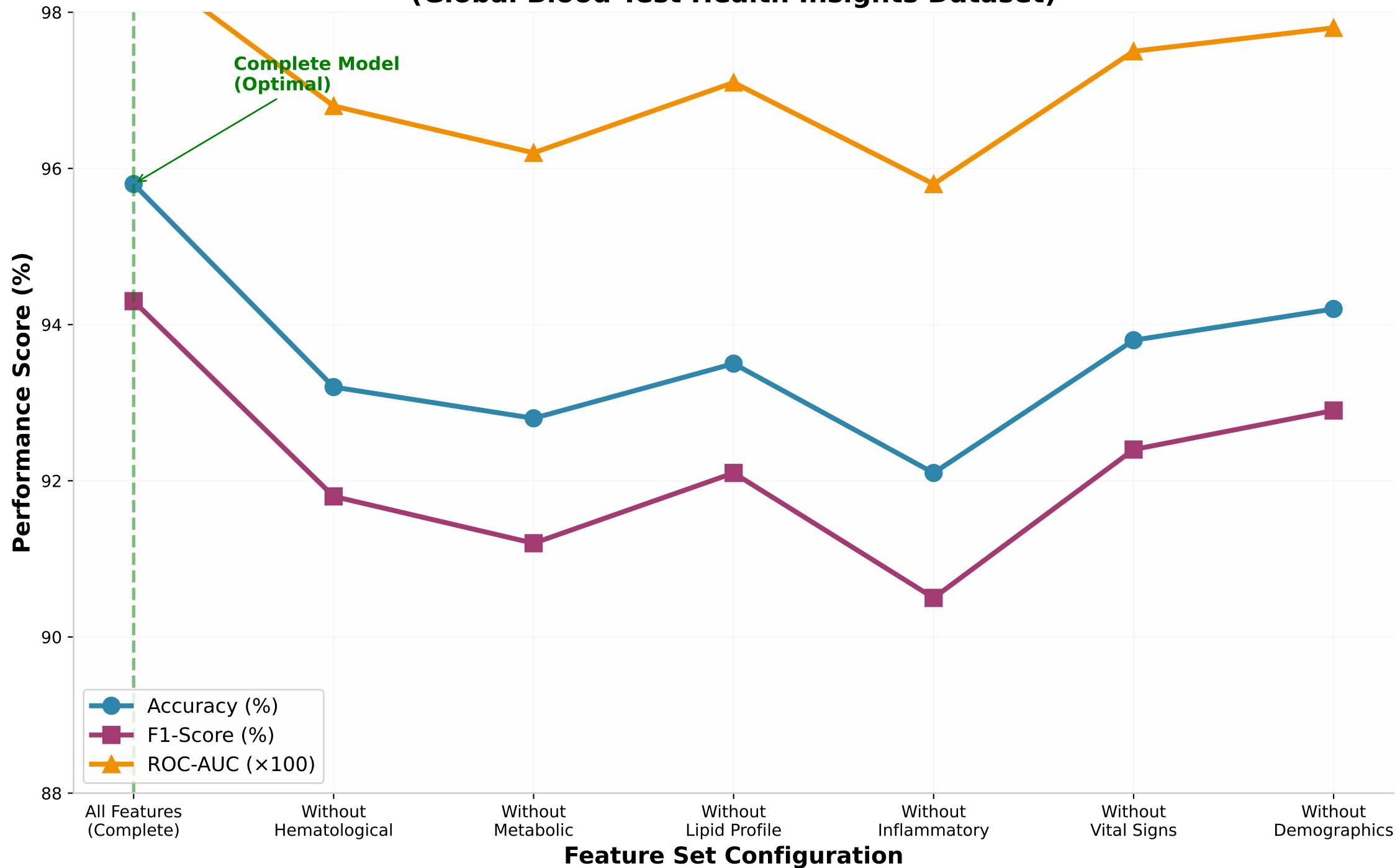
Figure 3.2 — Model Robustness Under Missing Feature Groups (Global Blood Test Health Insights Dataset)
