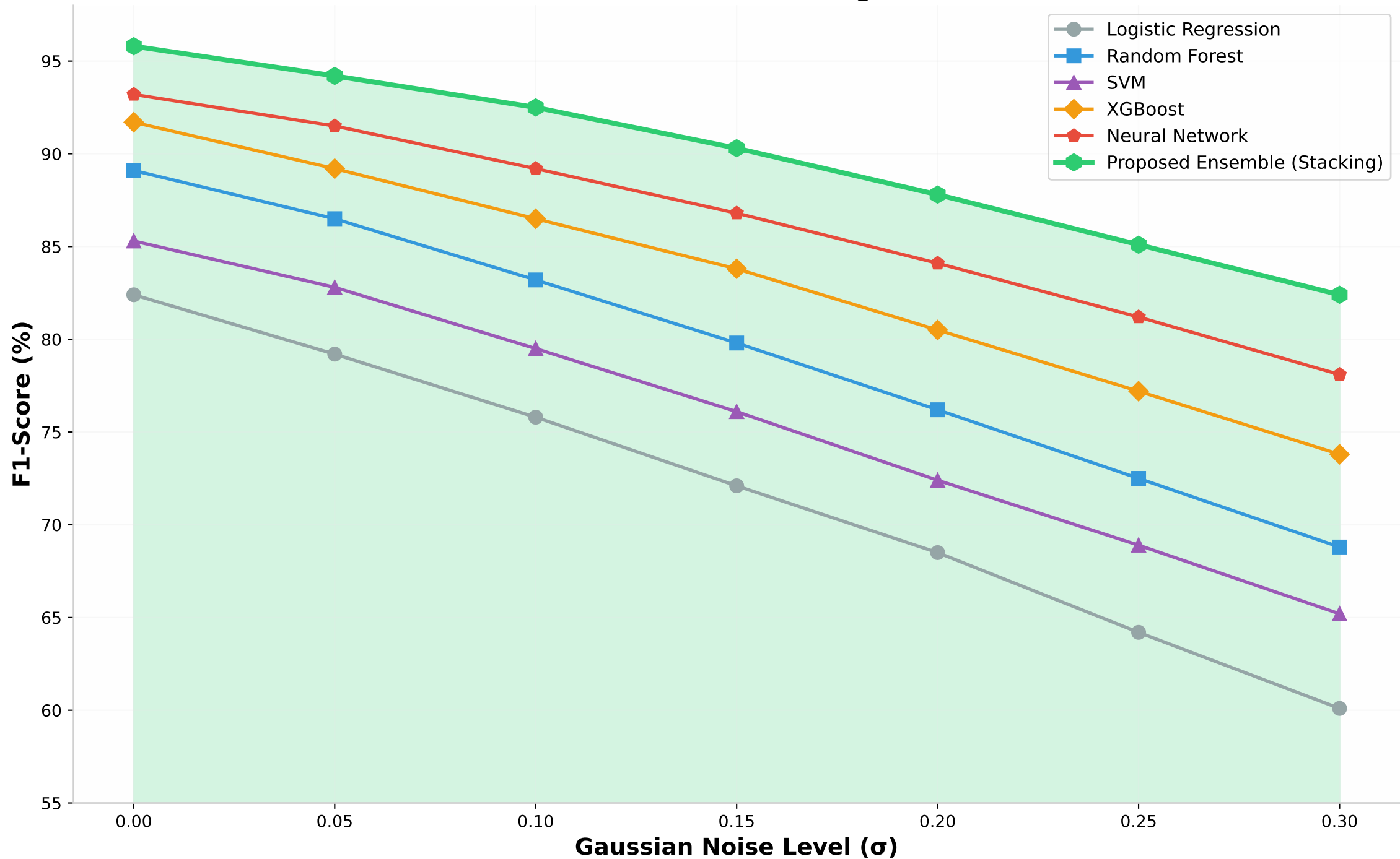
Figure 5.1 — Robustness Degradation Curves Under Increasing Data Noise (Global Blood Test Health Insights Dataset)
