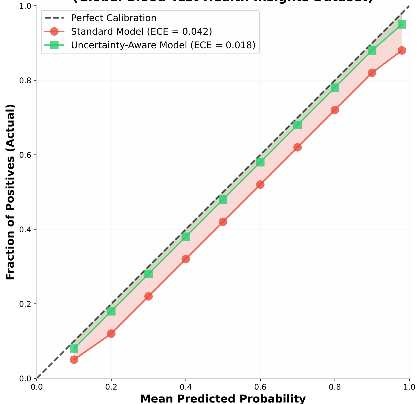
Figure 6.1 — Calibration / Reliability Diagram (Global Blood Test Health Insights Dataset)
