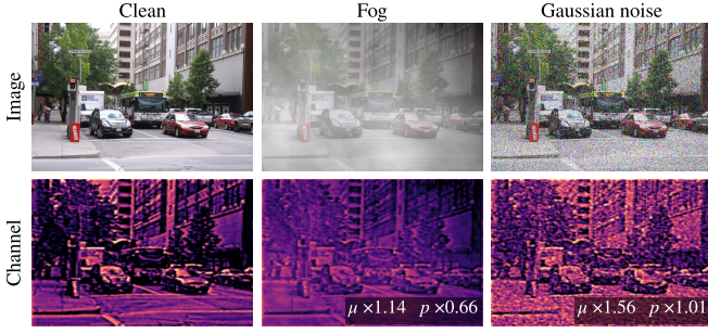
Fig. 1. A backbone channel of RT-DETRv2-R18 on one image. Top: clean image, image under fog and image under Gaussian noise. Bottom: the channel’s response maps, where brighter means a stronger response. Relative to the clean image, fog lowers the peak response p , and noise raises the mean response \mu .
