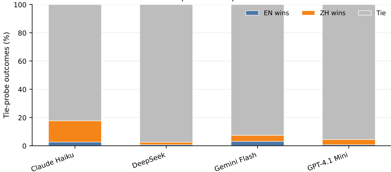
Translation-equivalent tie-probe outcomes
