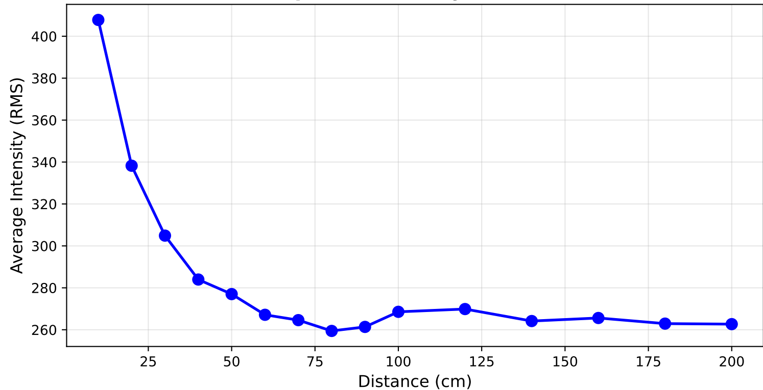
Microphone Intensity vs Distance
