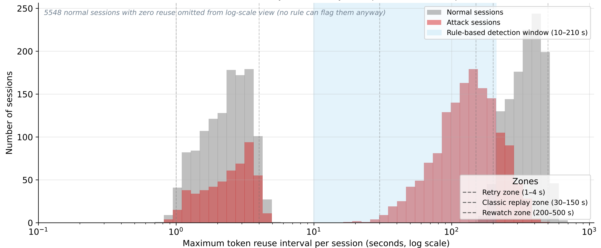
Reuse interval distribution by class — why a simple rule cannot separate
