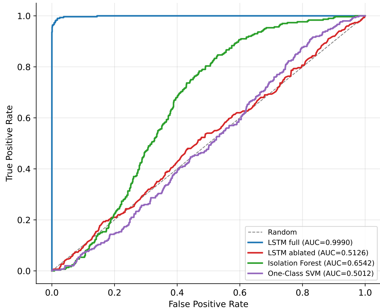
ROC curves — test set
