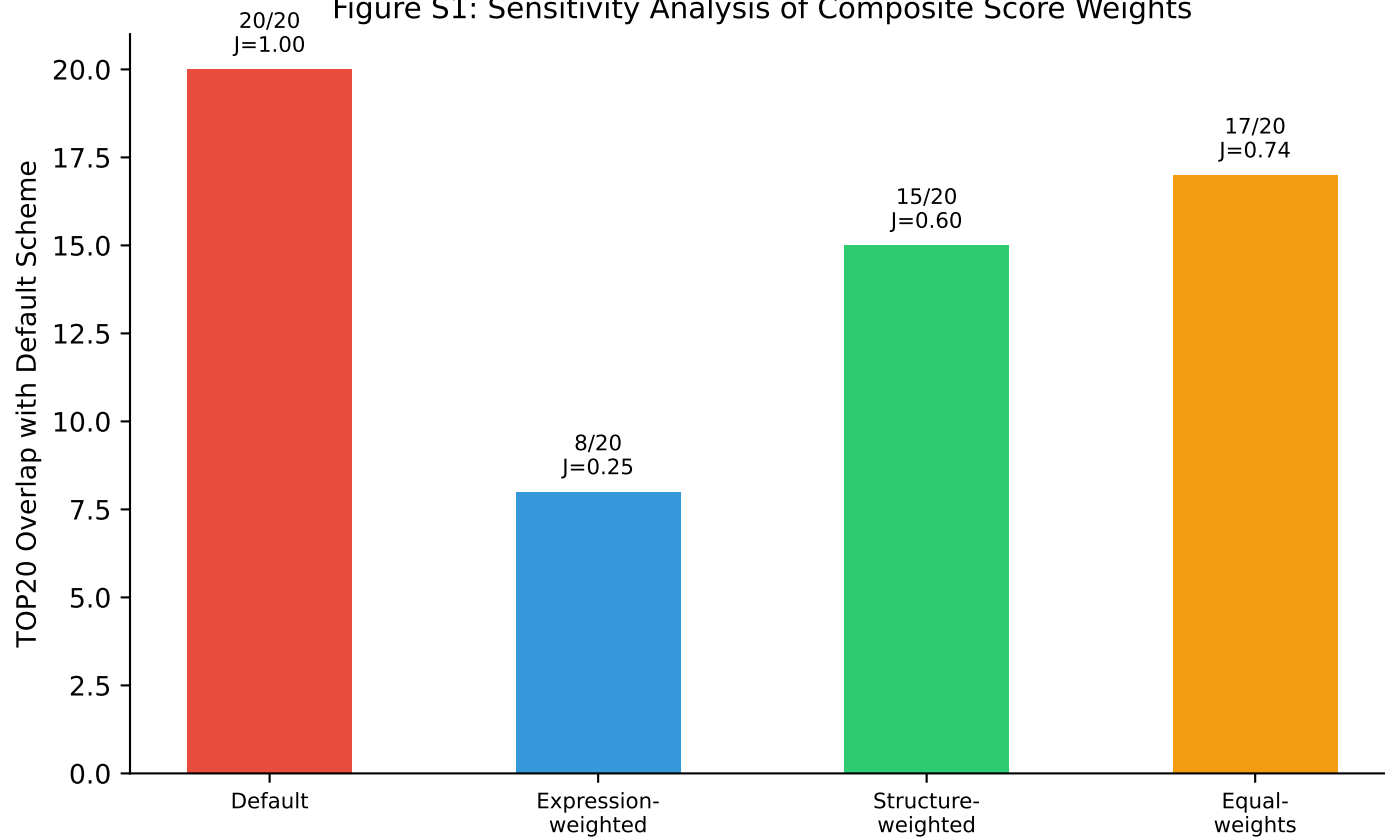
Figure S1: Sensitivity Analysis of Composite Score Weights
