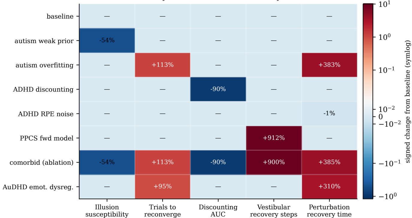
Lever effects stay confined to the modules they are wired into
