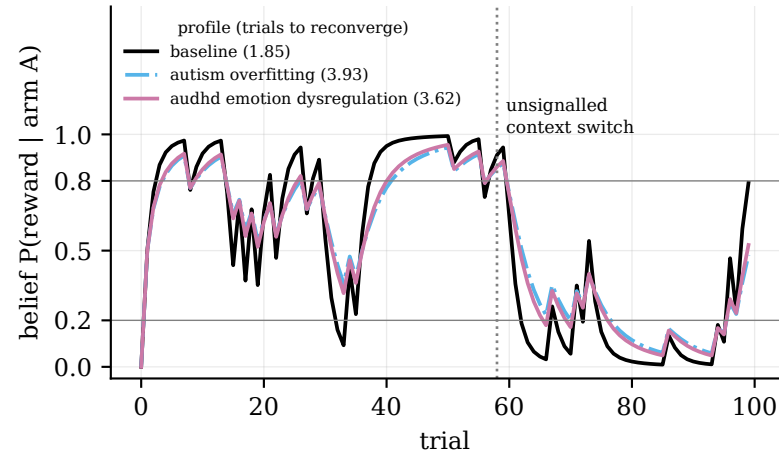
Volatility learning
