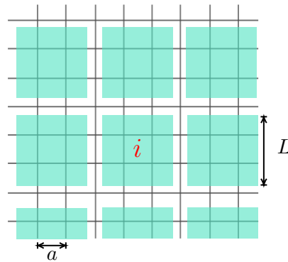
Figure 23: Coarse graining the lattice
