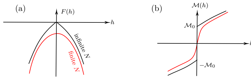
Figure 13: (a) Free energy and (b) Magnetisation behaviour in finite N and thermodynamic limit for T < T_c .
