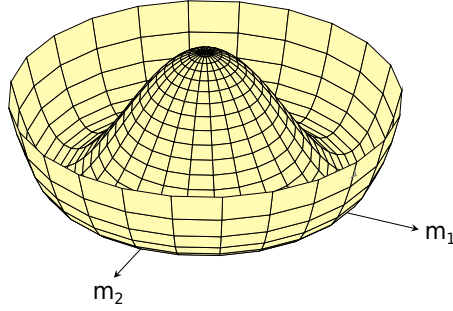
Figure 28: Homogenous part of the Landau functional for n = 2 . This is the famous Mexican hat potential . The minima is spherically symmetric.
