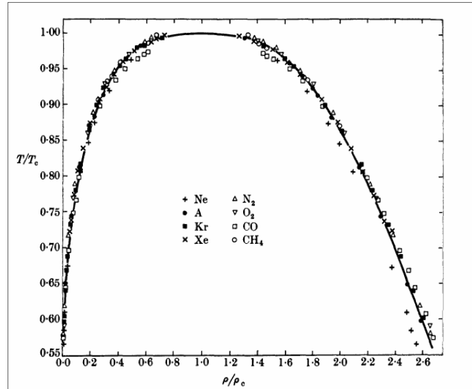
Figure 7: The Guggenheim plot for different gases with reduced parameter, showing that the trend follows a universal function (Source: Guggenheim (1945) [2]).
