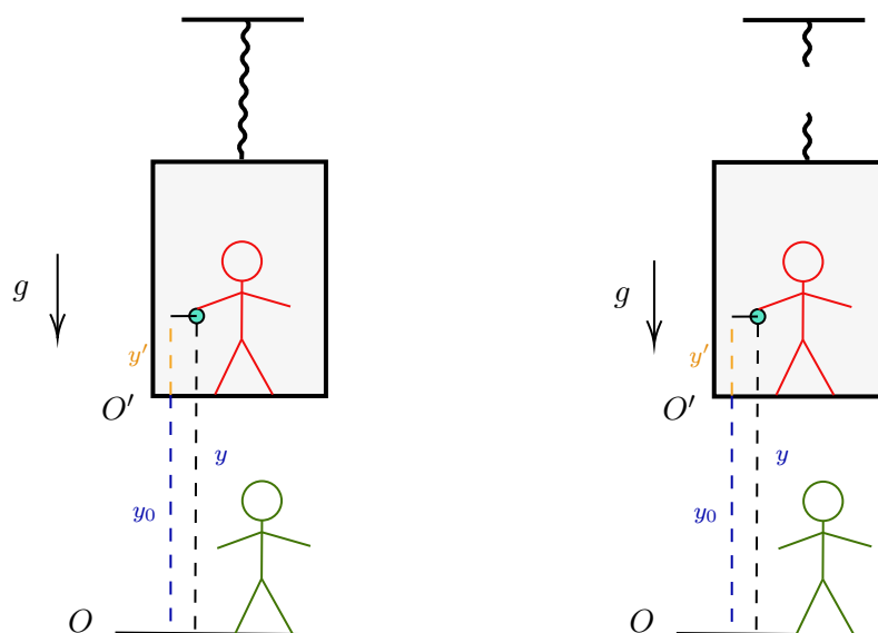
Case 1 : Hanging lift
