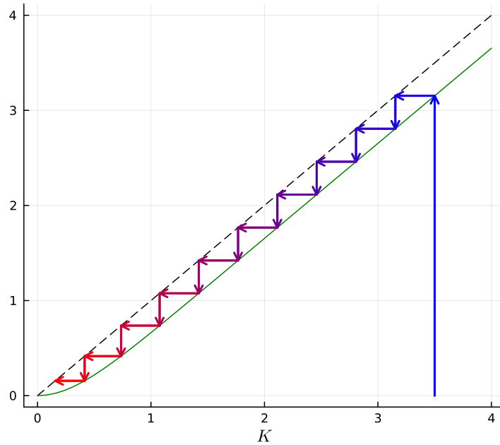
Figure 31: The decimation process. Starting from K_0 = 3.5 , we map it onto the curve K' = \frac{1}{2} \ln \cosh 2K and repeat the process. The black dashed line represents K' = K line while the green line represents K' = \frac{1}{2} \ln \cosh 2K line. The process converges to K^* = 0
