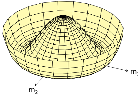
Figure 27: Homogenous part of the Landau functional for n = 2 . This is the famous Mexican hat potential .
