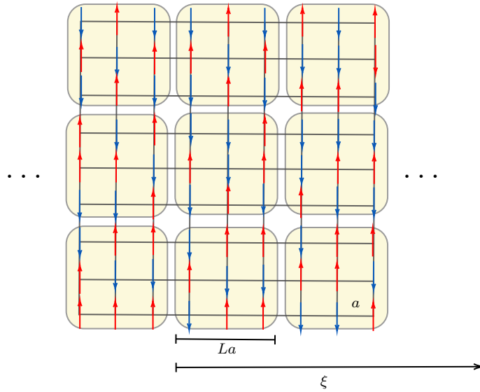
Figure 28: Kadanoff's block-spin construction
