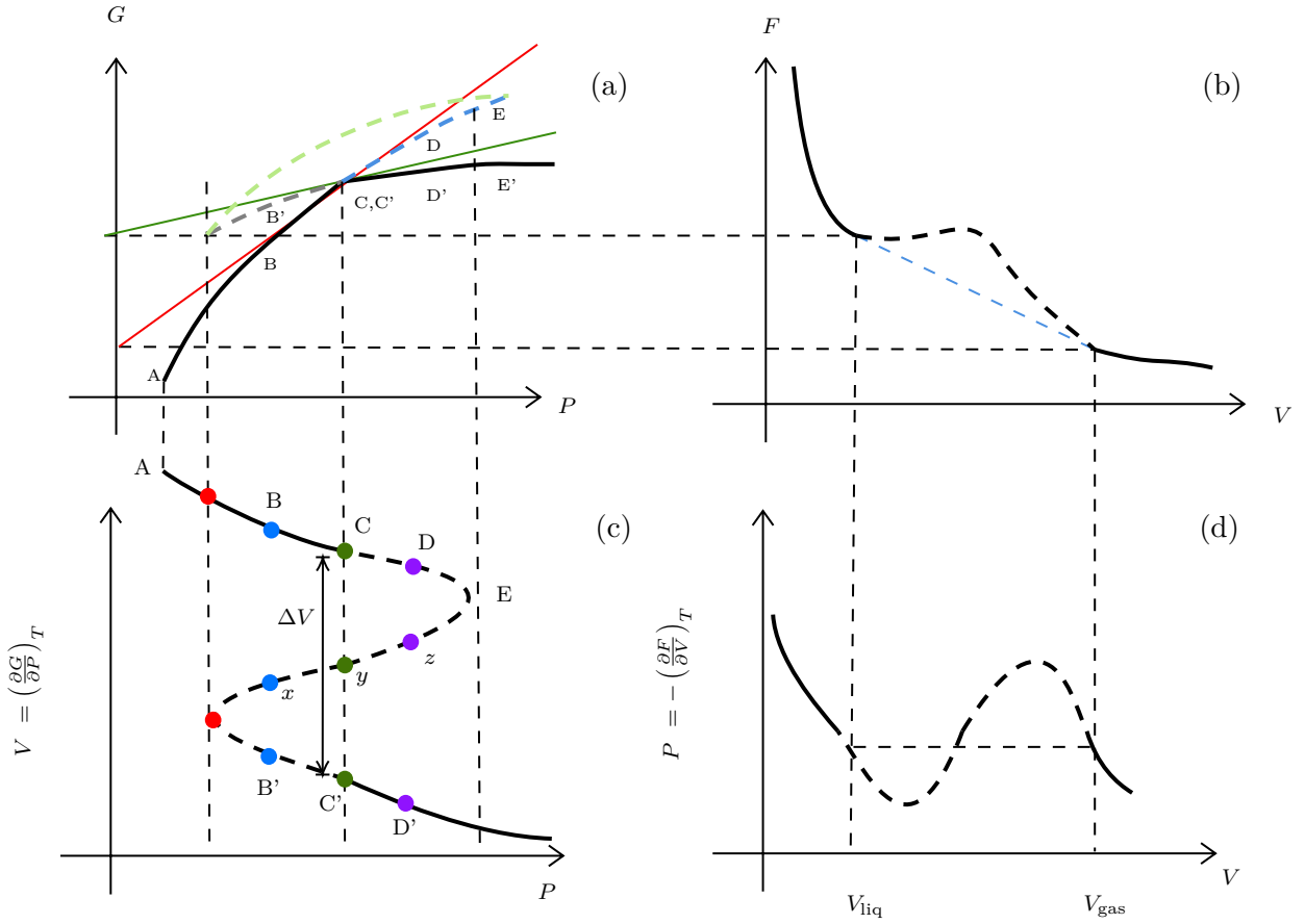
Figure 3: Plot of different quantities for T < T_c
