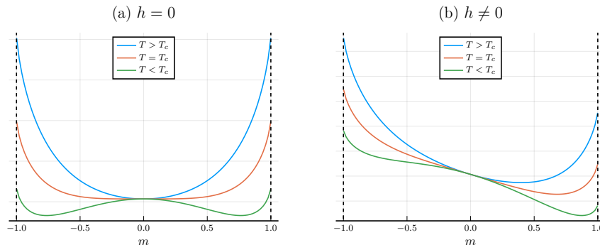
Figure 15: \mathcal{L} vs. m at different temperature regimes.
