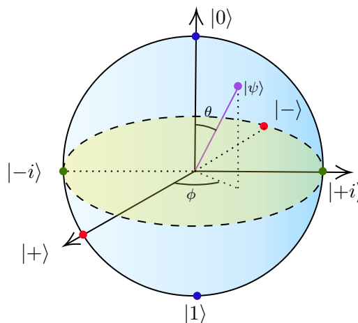
Figure 10: The Bloch Sphere. All important states lying at special points have been shown. An arbitrary state |\psi\rangle is also shown at a point (\theta, \phi)
