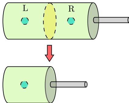
Figure 8: Demonstration of Landauer's Principle
