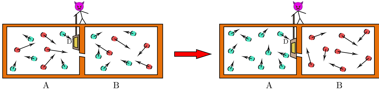
Figure 9: Schematic of the Maxwell's demon. The red particles are fast moving while blue particles are slow moving. The demon is shown holding the trap-door!
