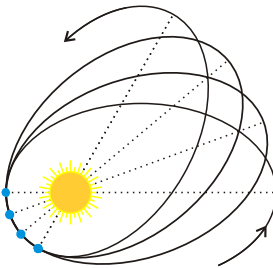
Figure 9: Diagram showing the perihelion shift of a planet
