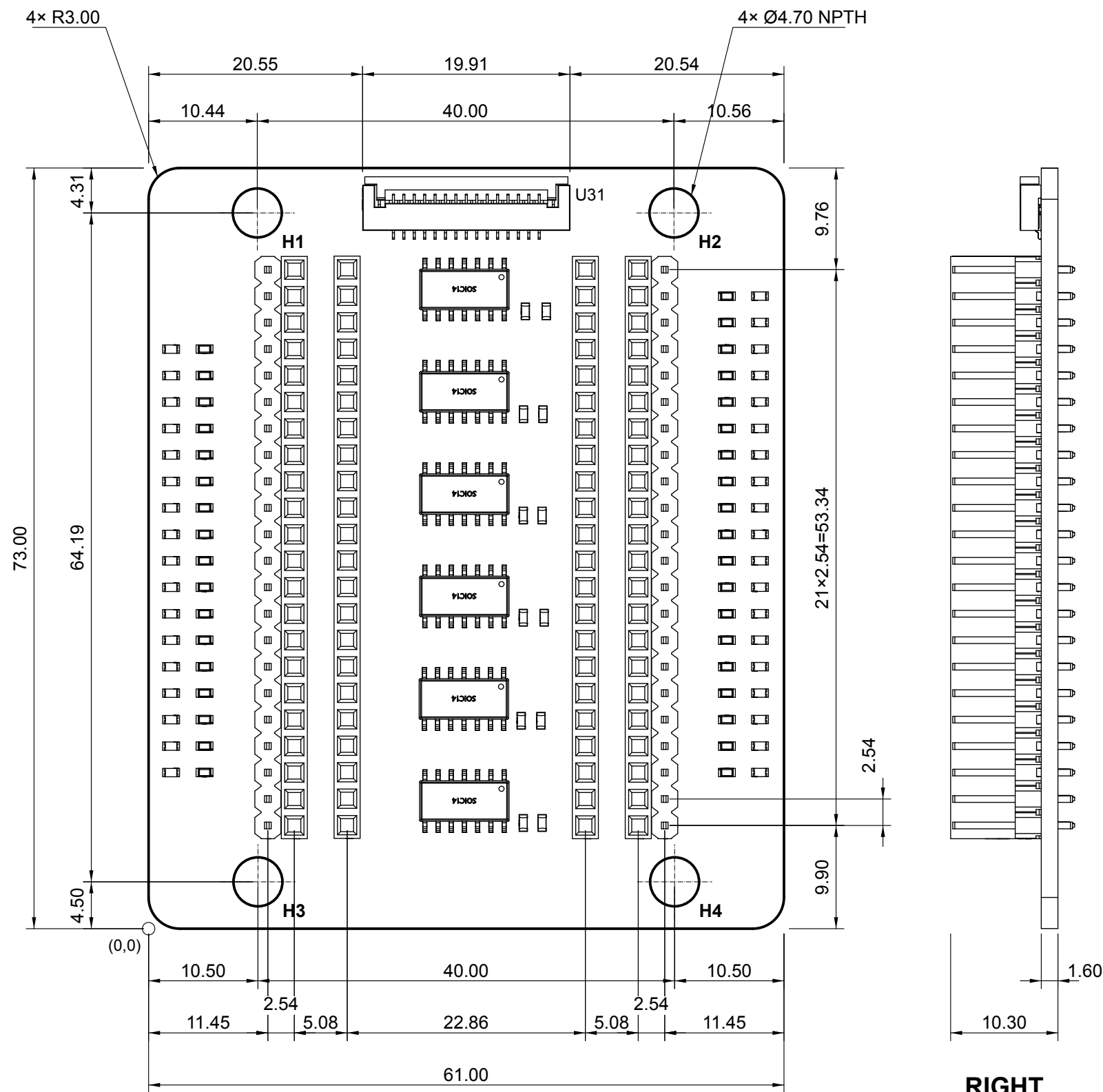
TOP VIEW
