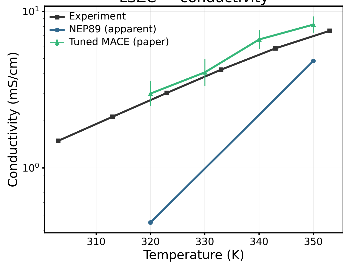
LSZC — conductivity
