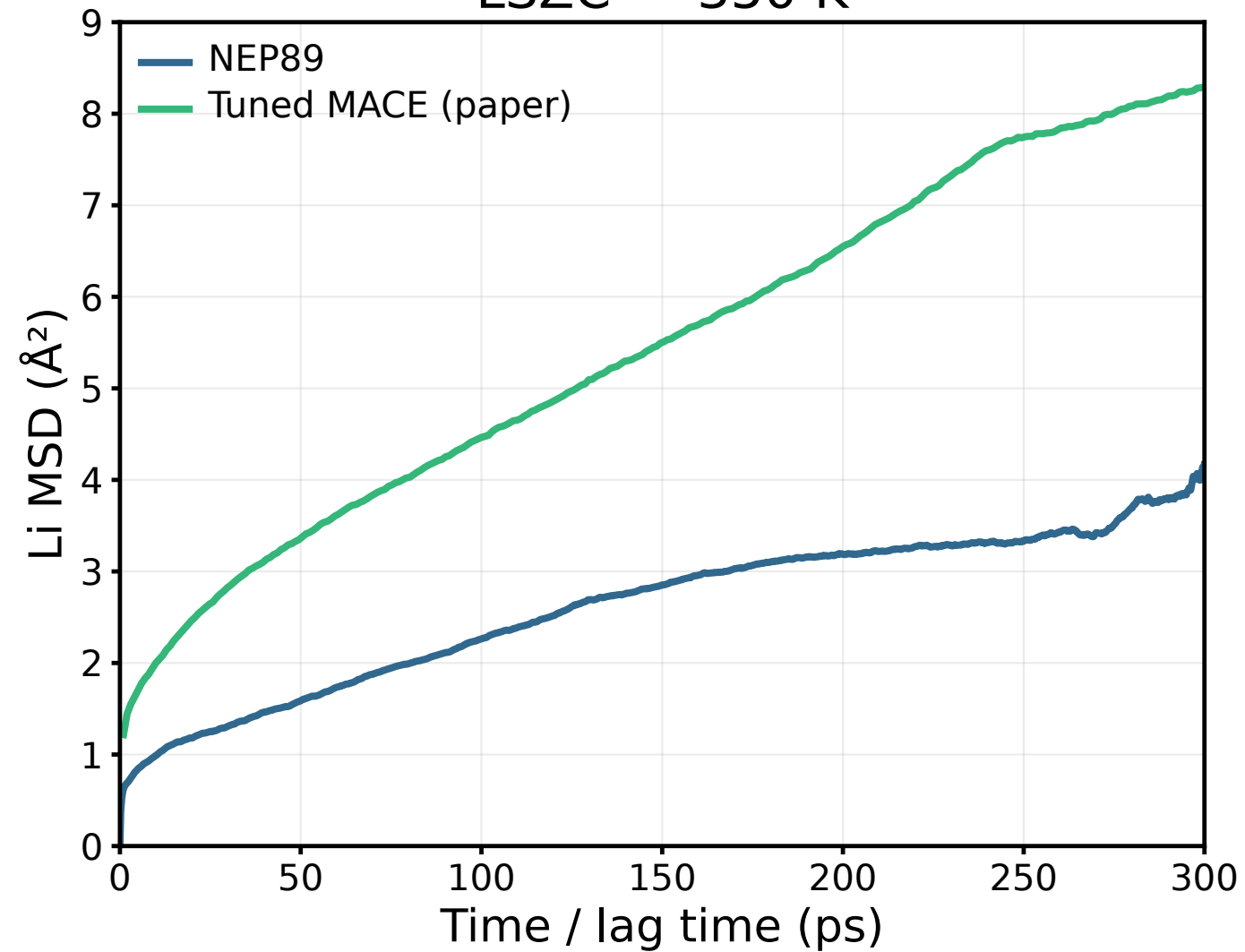
LSZC — 350 K
