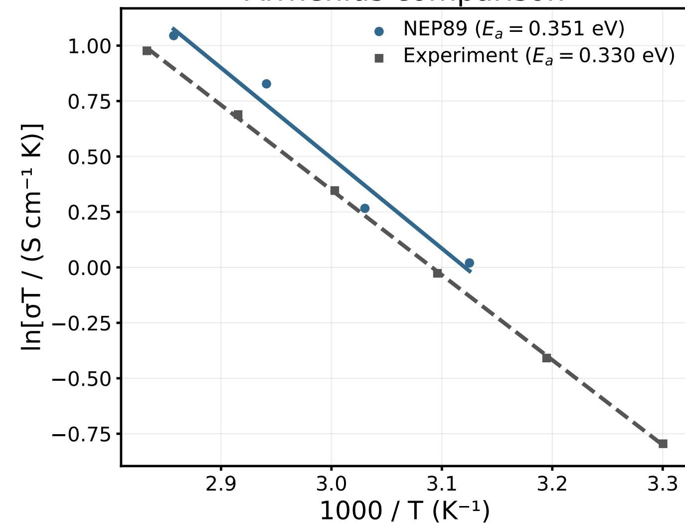
Arrhenius comparison
