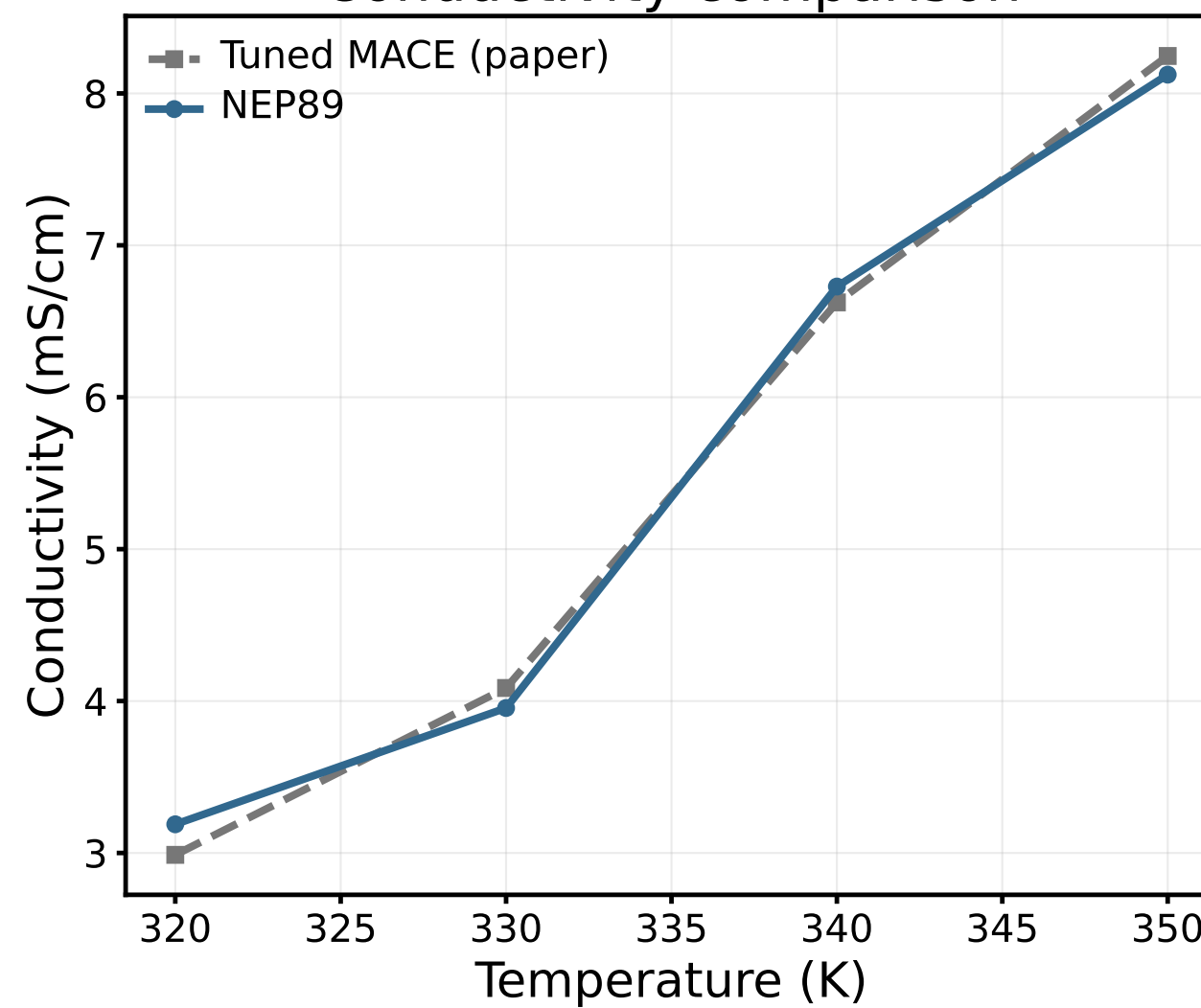
Conductivity comparison
