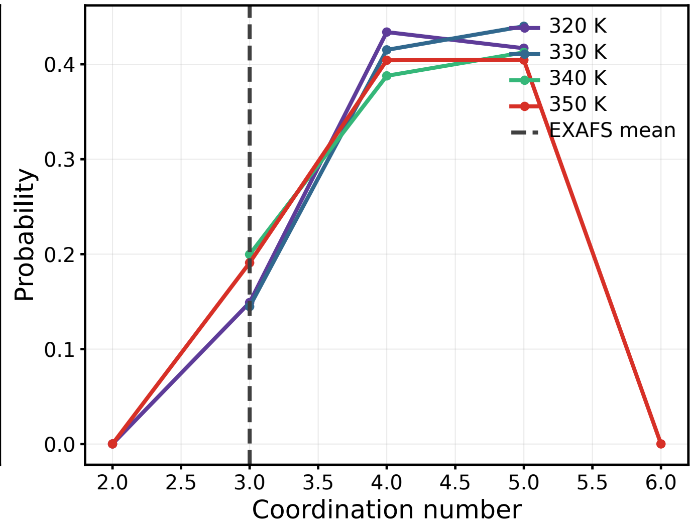
Zr-Cl coordination
