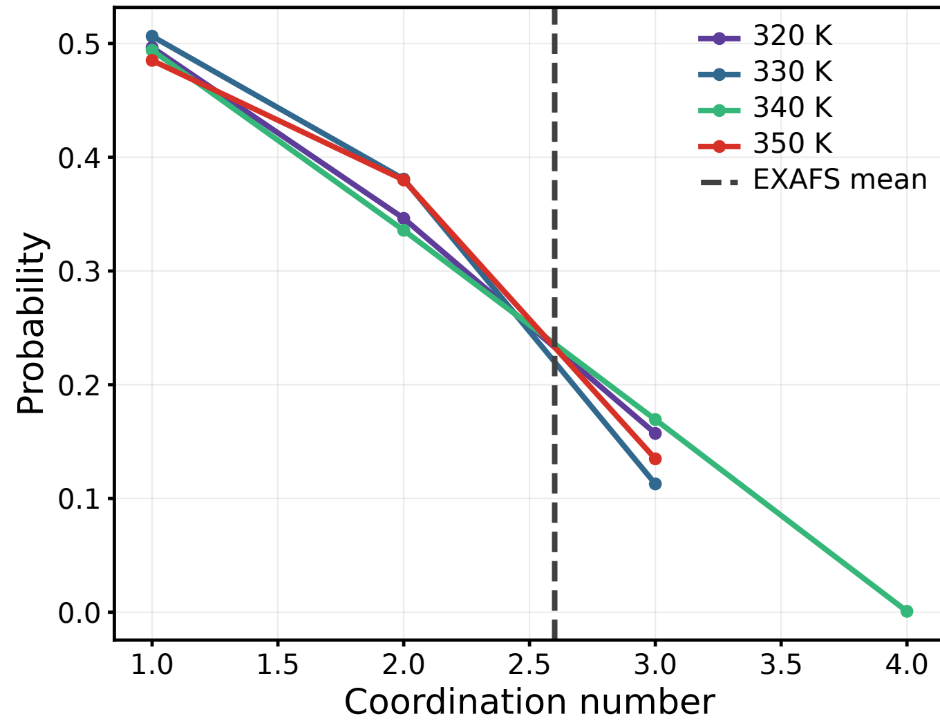
Zr-O coordination
