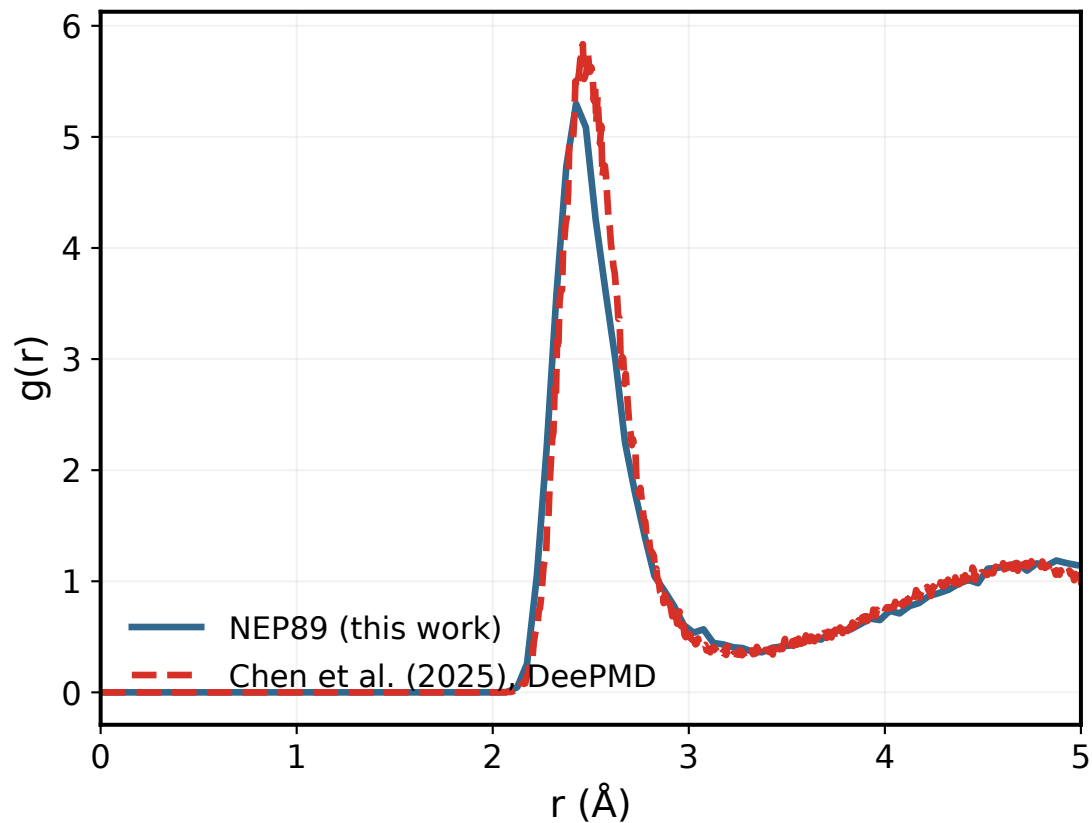
Li-S radial distribution
