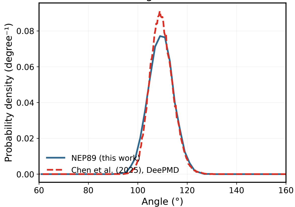
S-P-S angle distribution
