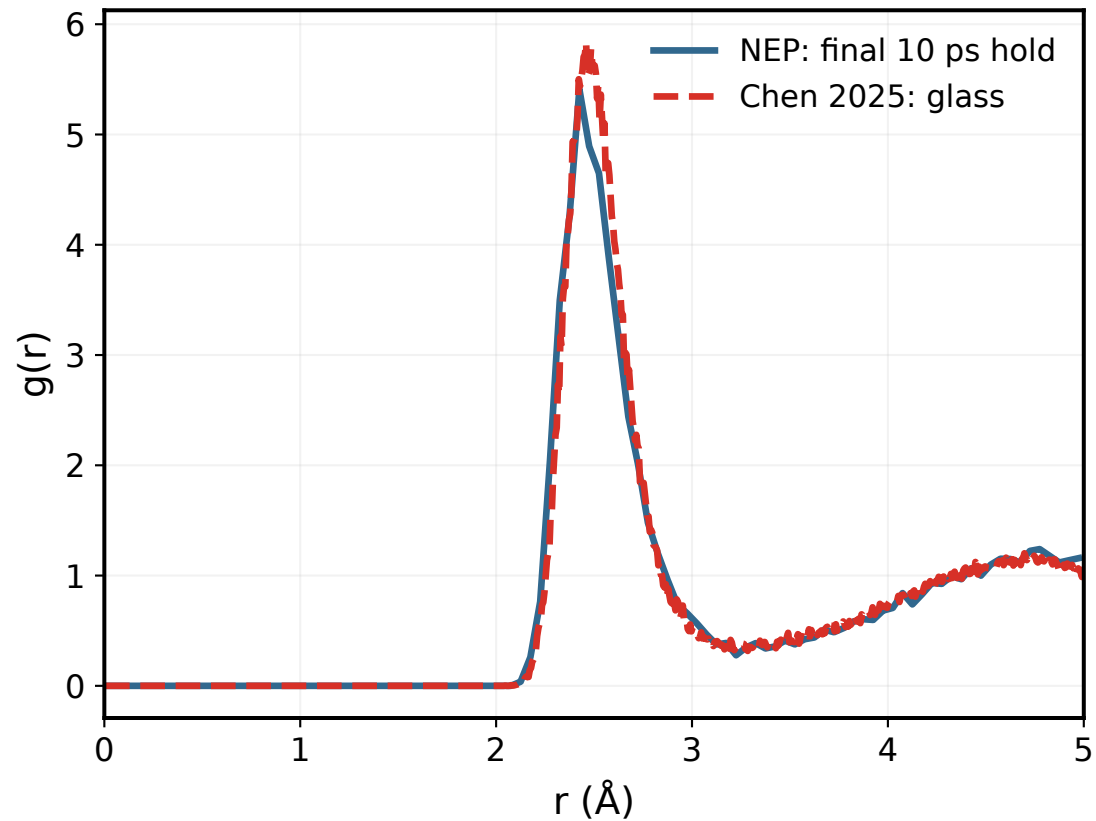
Li-S RDF
