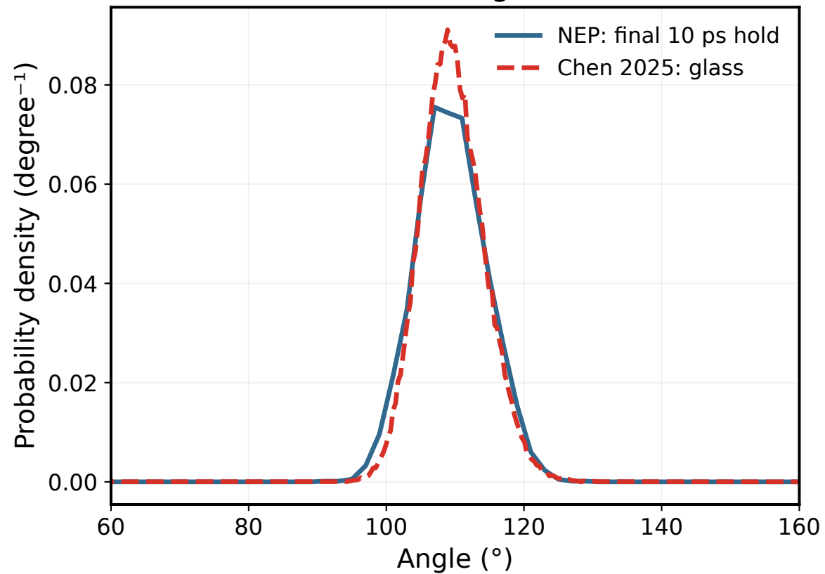
S-P-S angles
