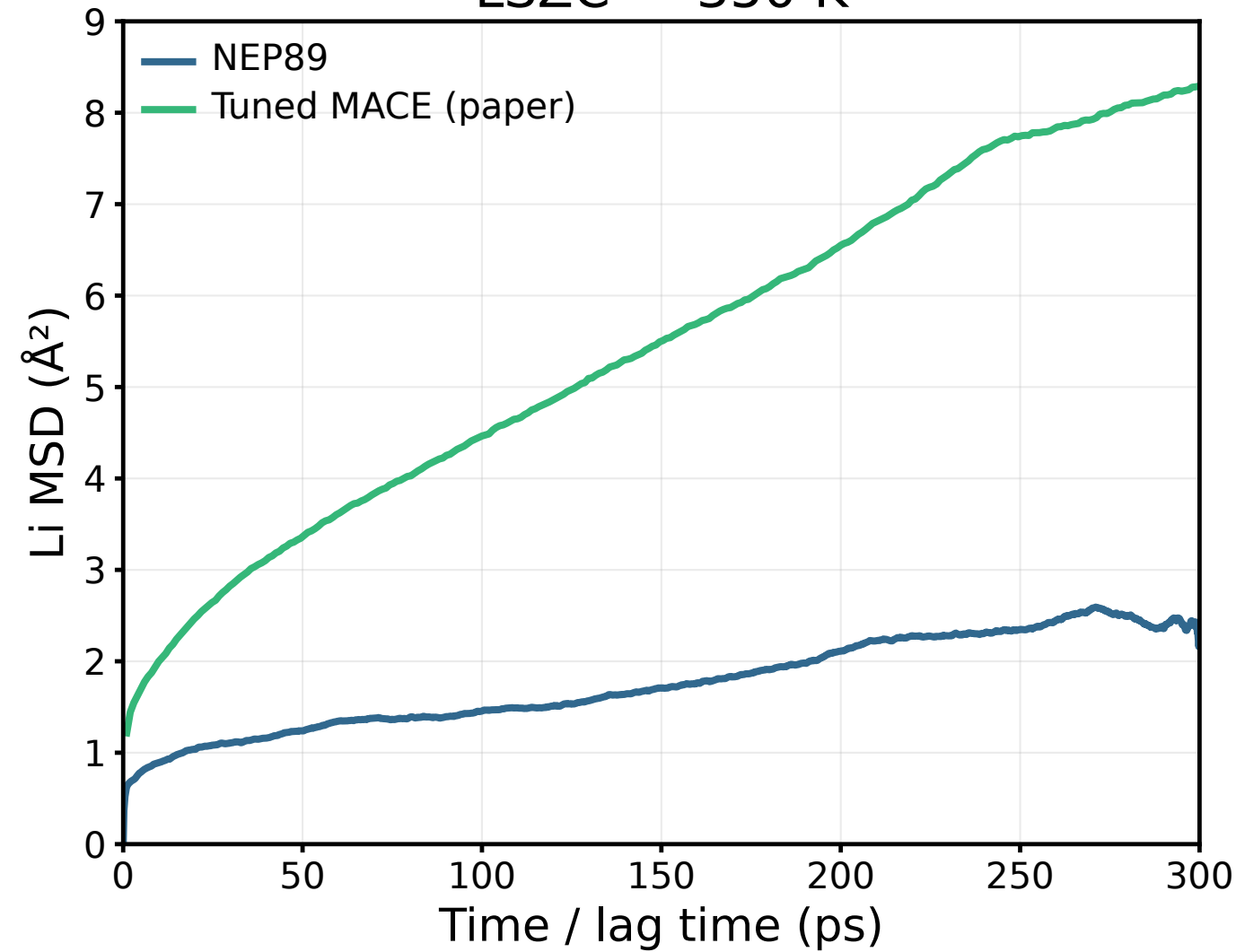
LSZC — 350 K
