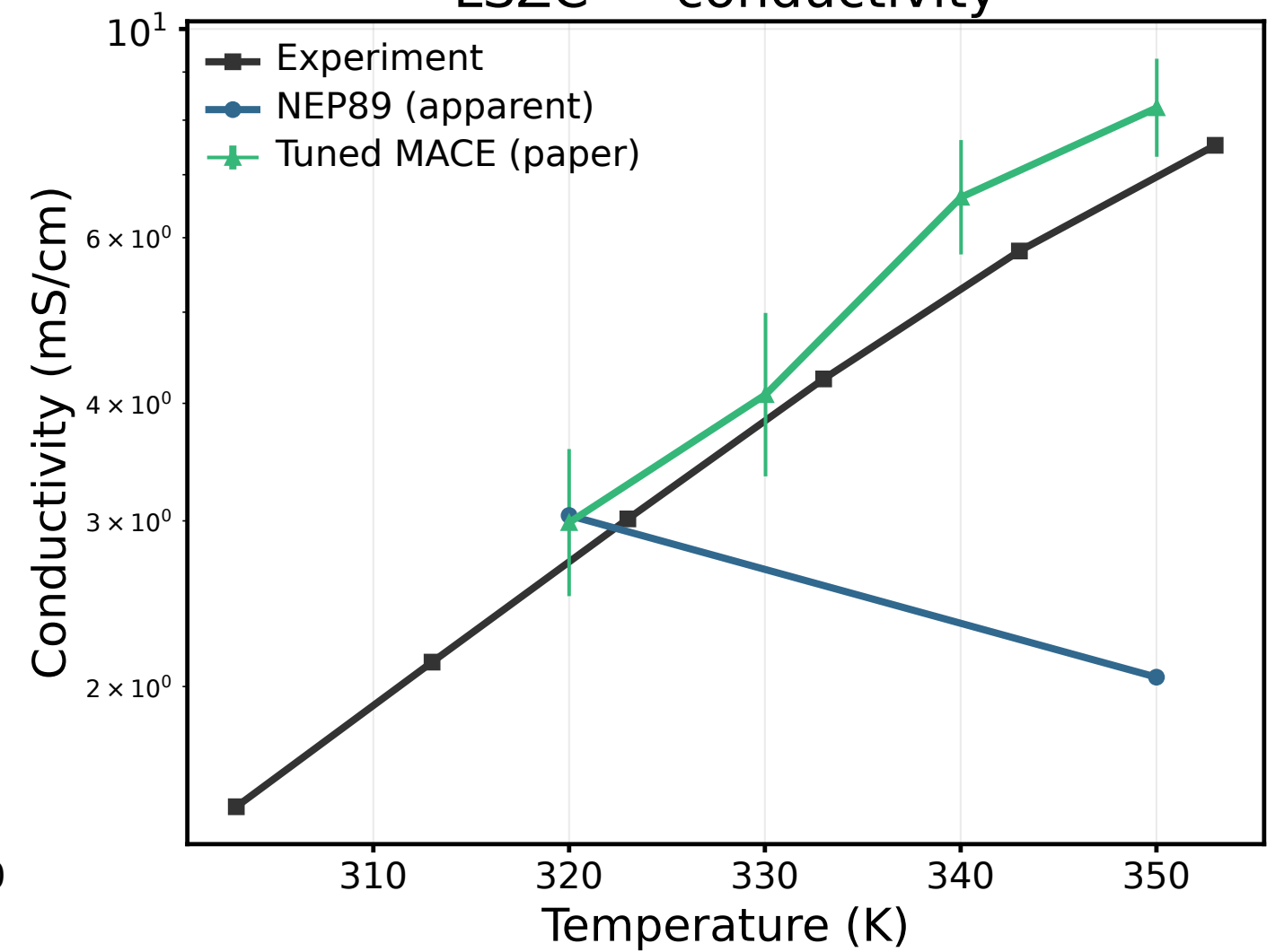
LSZC — conductivity
