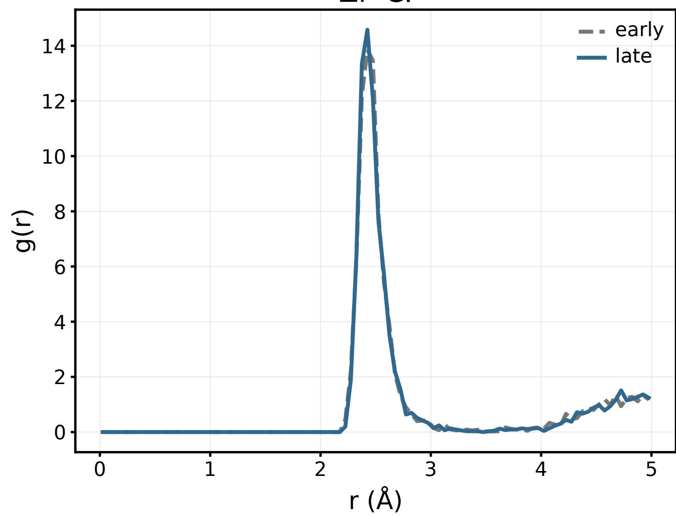
Zr-Cl
