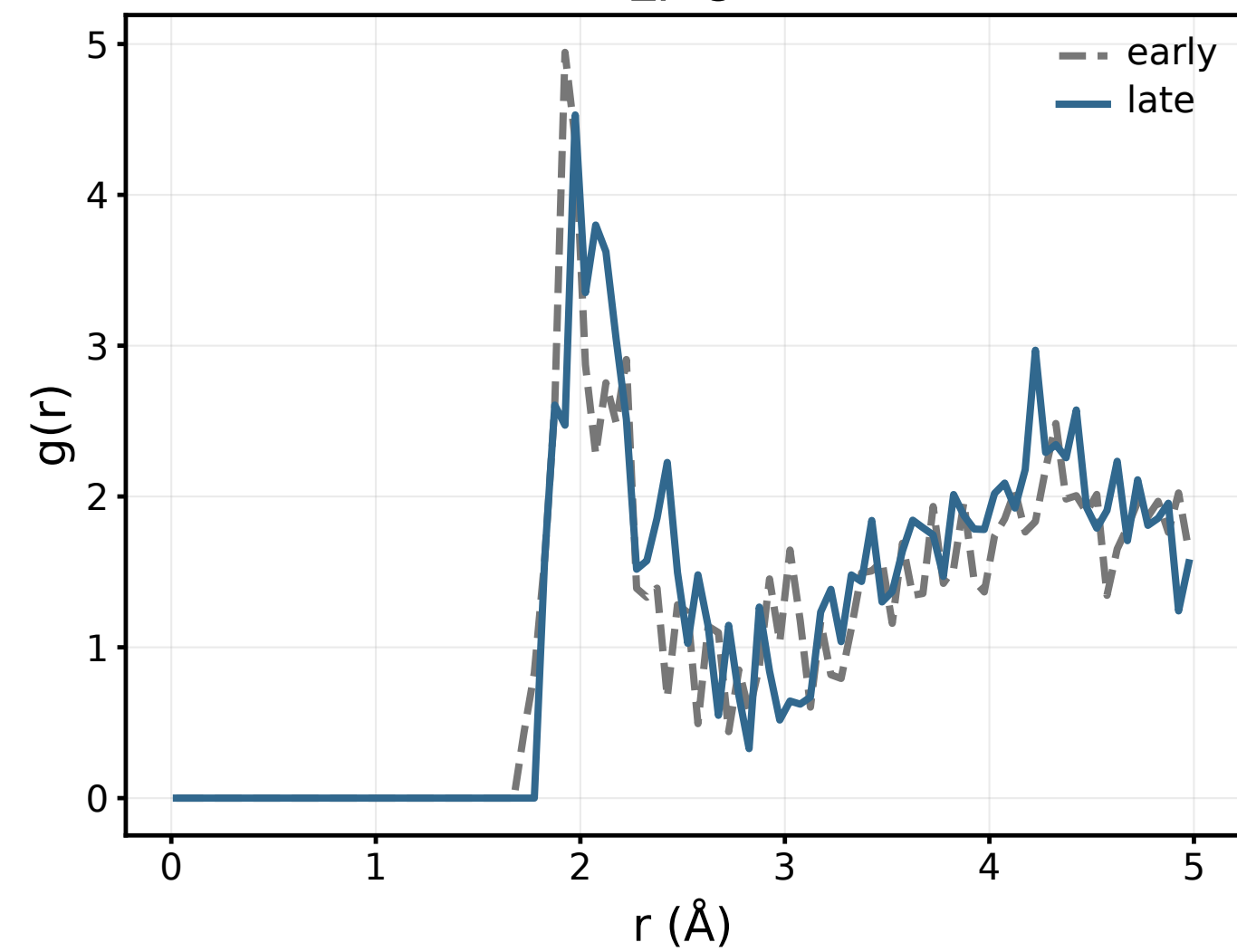
Zr-O
