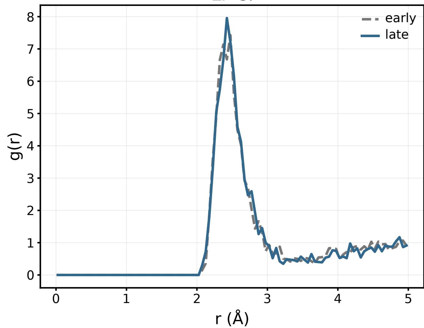
Zr-Cl
