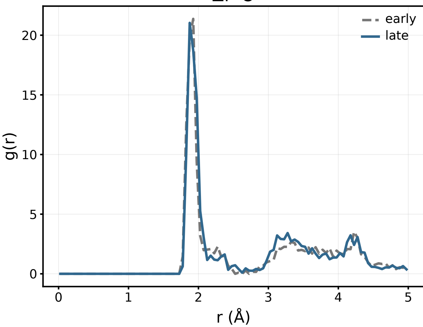
Zr-O
