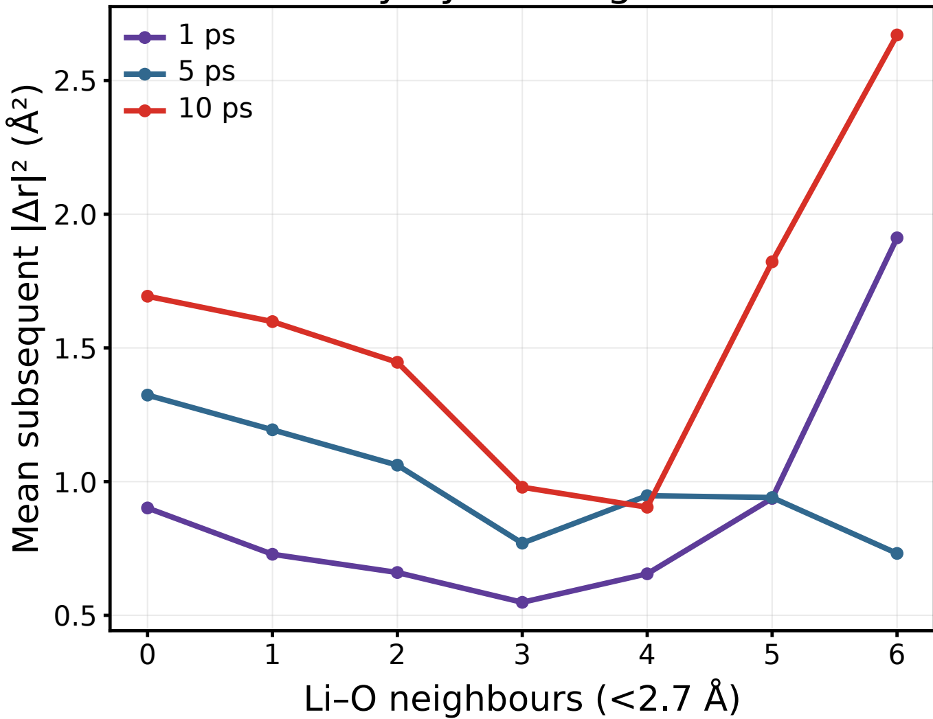
Mobility by starting Li-O CN
