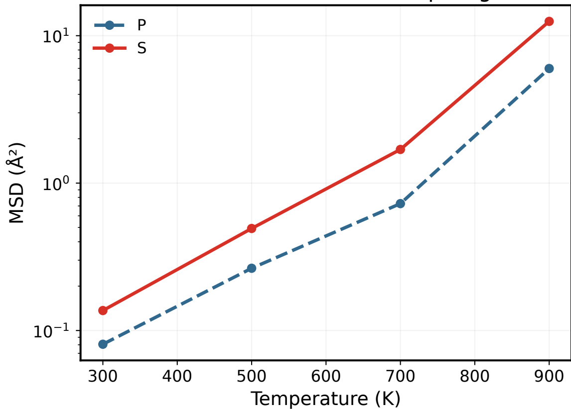
Framework motion at 80 ps lag
