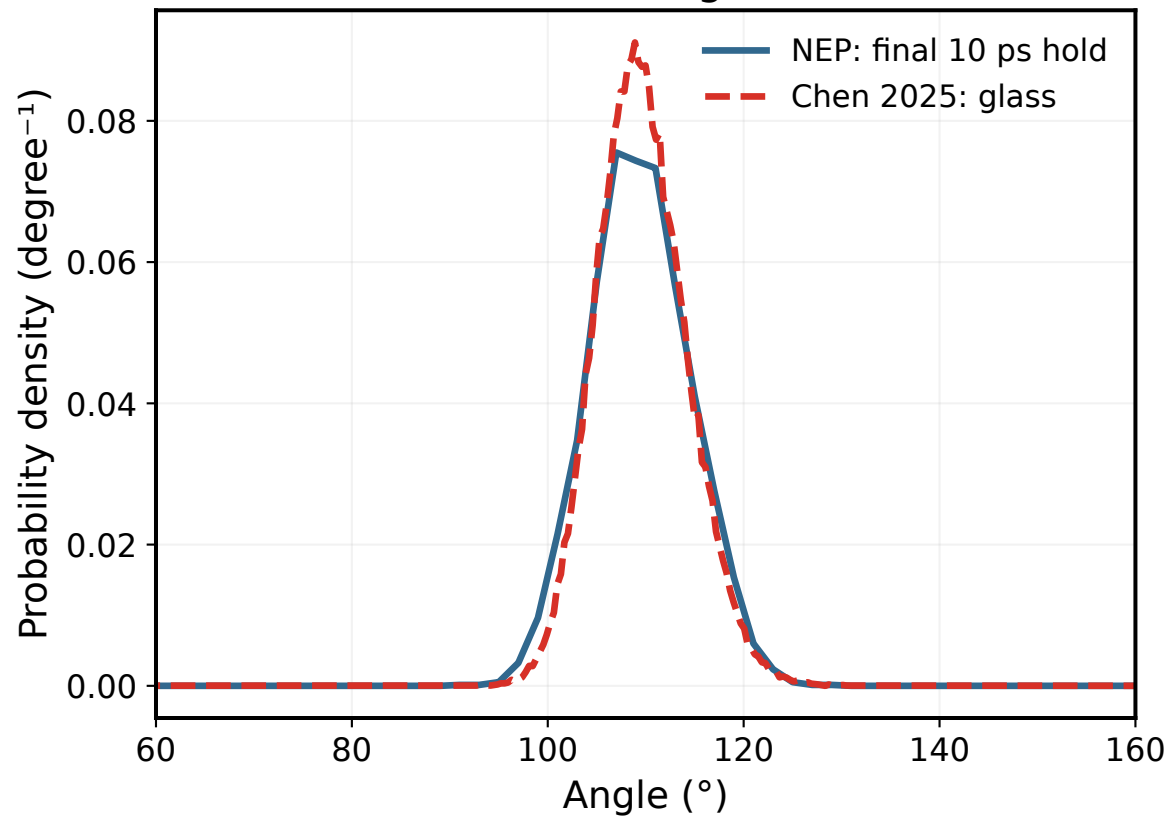
S-P-S angles
