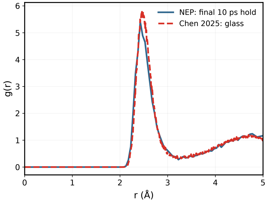
Li-S RDF
