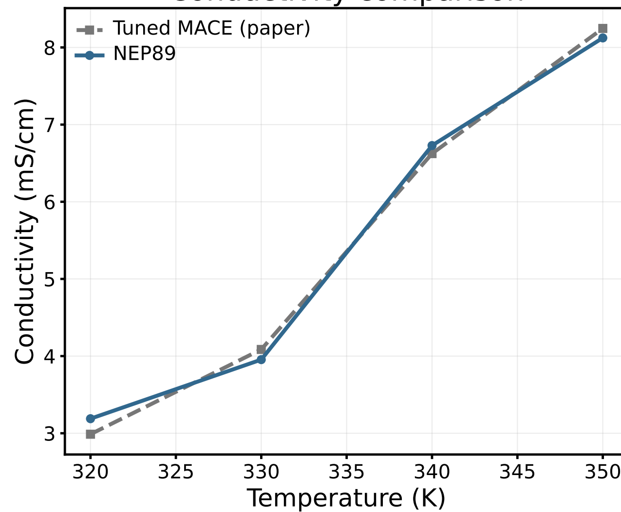
Conductivity comparison
