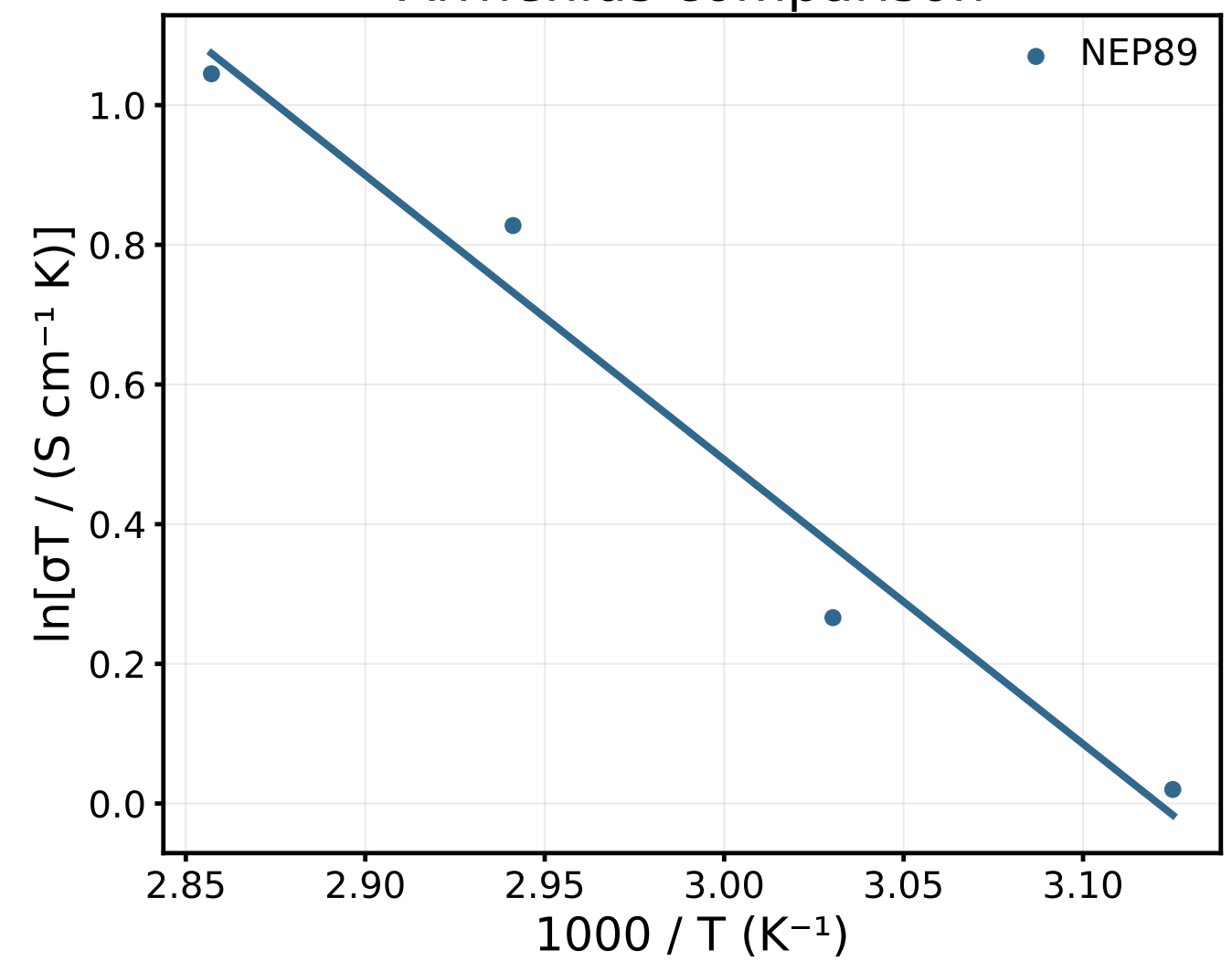
Arrhenius comparison
