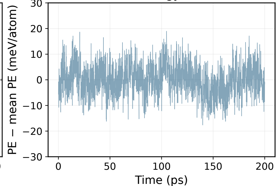
NEP89: NVT energy fluctuations
