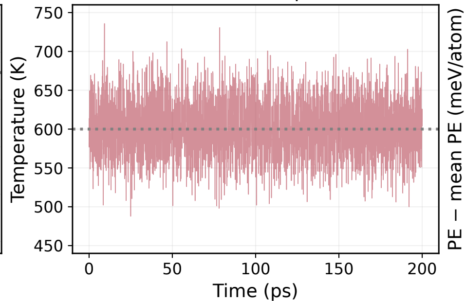
NEP89: NVT temperature
