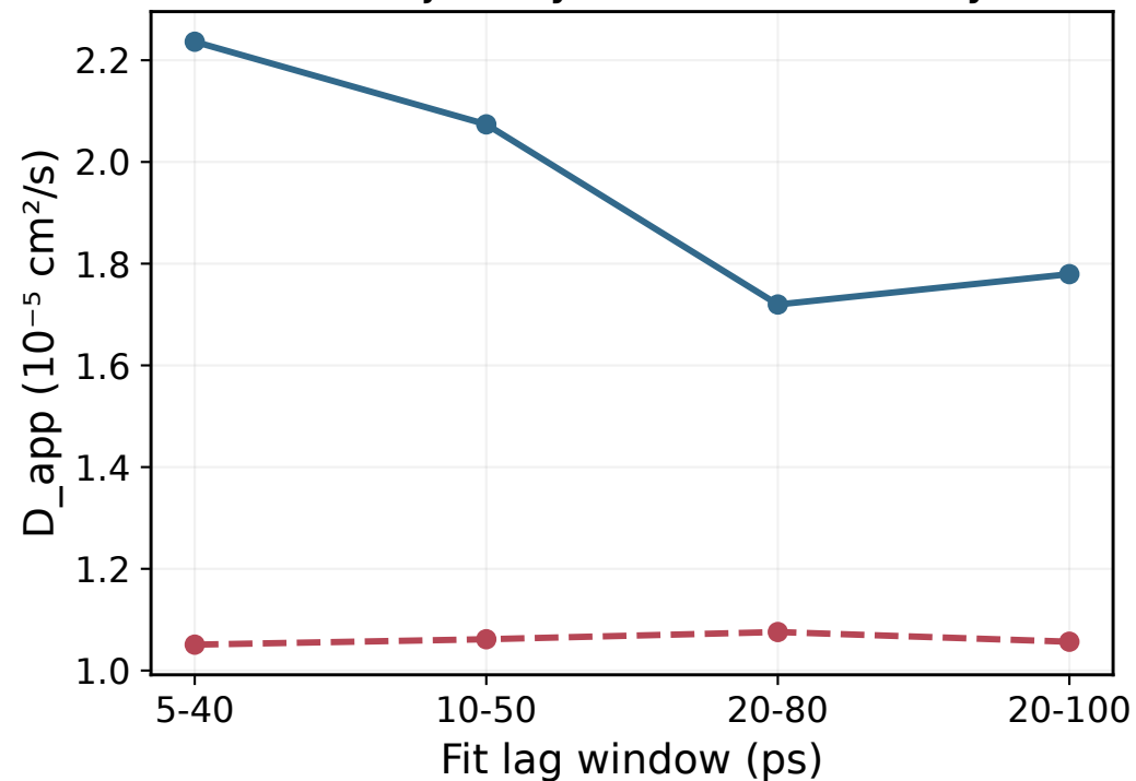
Li and framework motion
