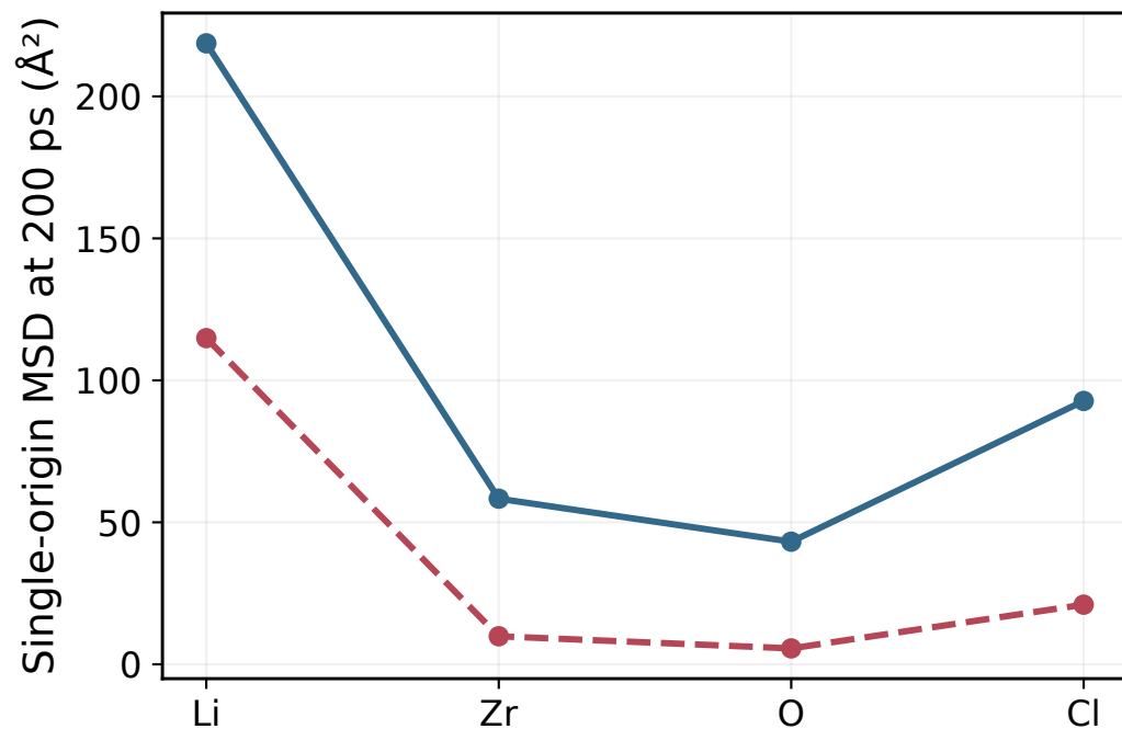
Li and framework motion
