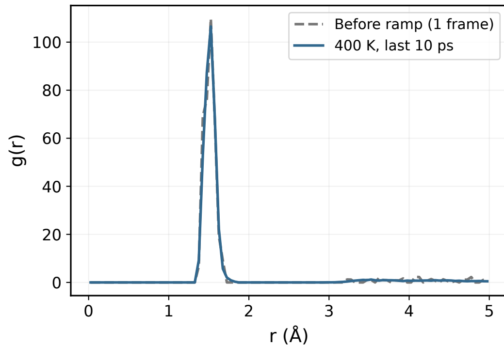
Zr-Cl
