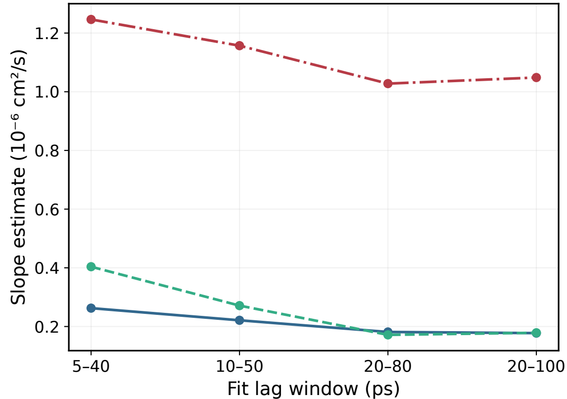
Window sensitivity (full trajectory)
