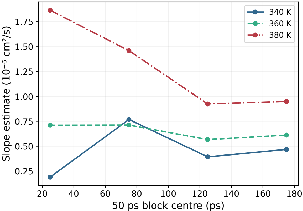
Within-trajectory blocks (5-20 ps fit)
