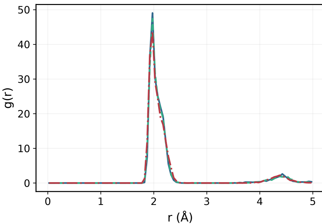
Zr-O
