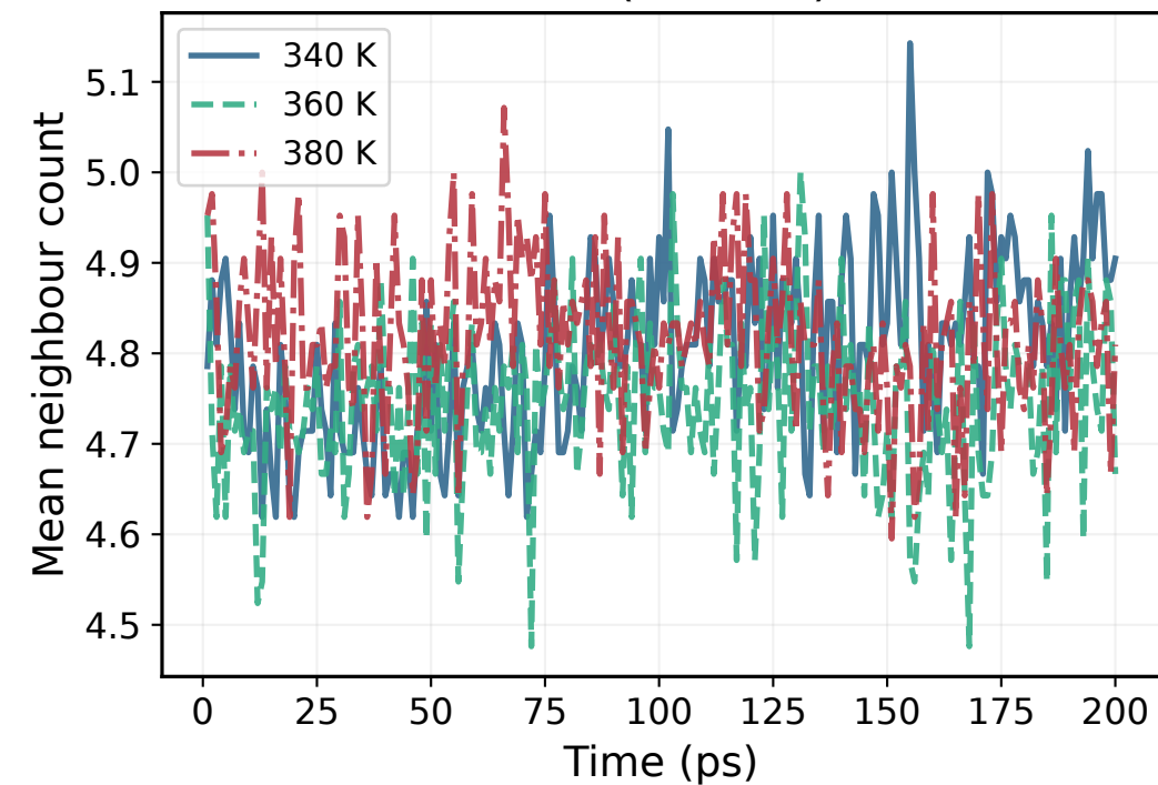
Zr-O ( < 2.6 \text{ \AA} )
