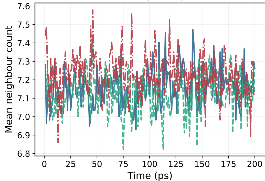
Cl-Cl ( < 4 \text{ \AA} )
